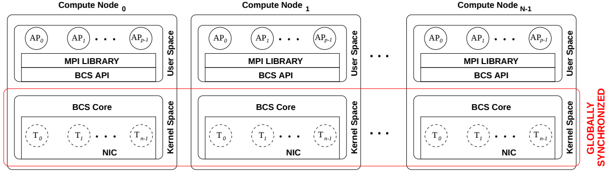
Figure 3: BCS-MPI Overview
