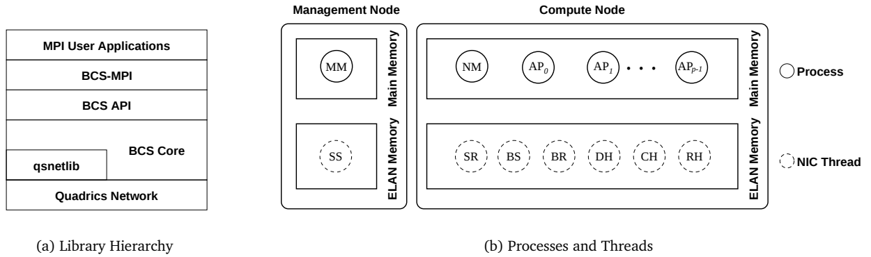
Figure 4: BCS-MPI Architecture
