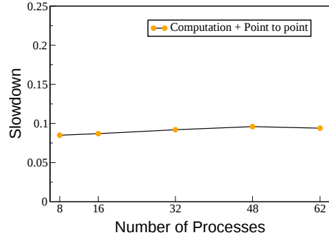
(d) Computation and Nearest-neighbor Communication: 10 ms granularity, 4 neighbors and 4KB messages
