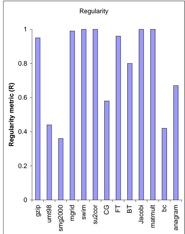
Figure 4: Regularity metric
